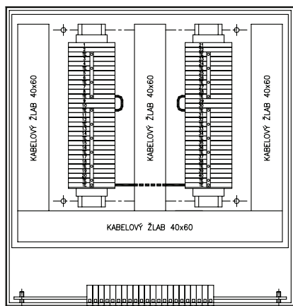
X341X2 DEP typ1 X341X2/JB DEP typ2
