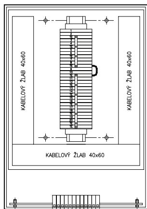
X340X2 DEP typ3 X340X2/JB DEP typ4
